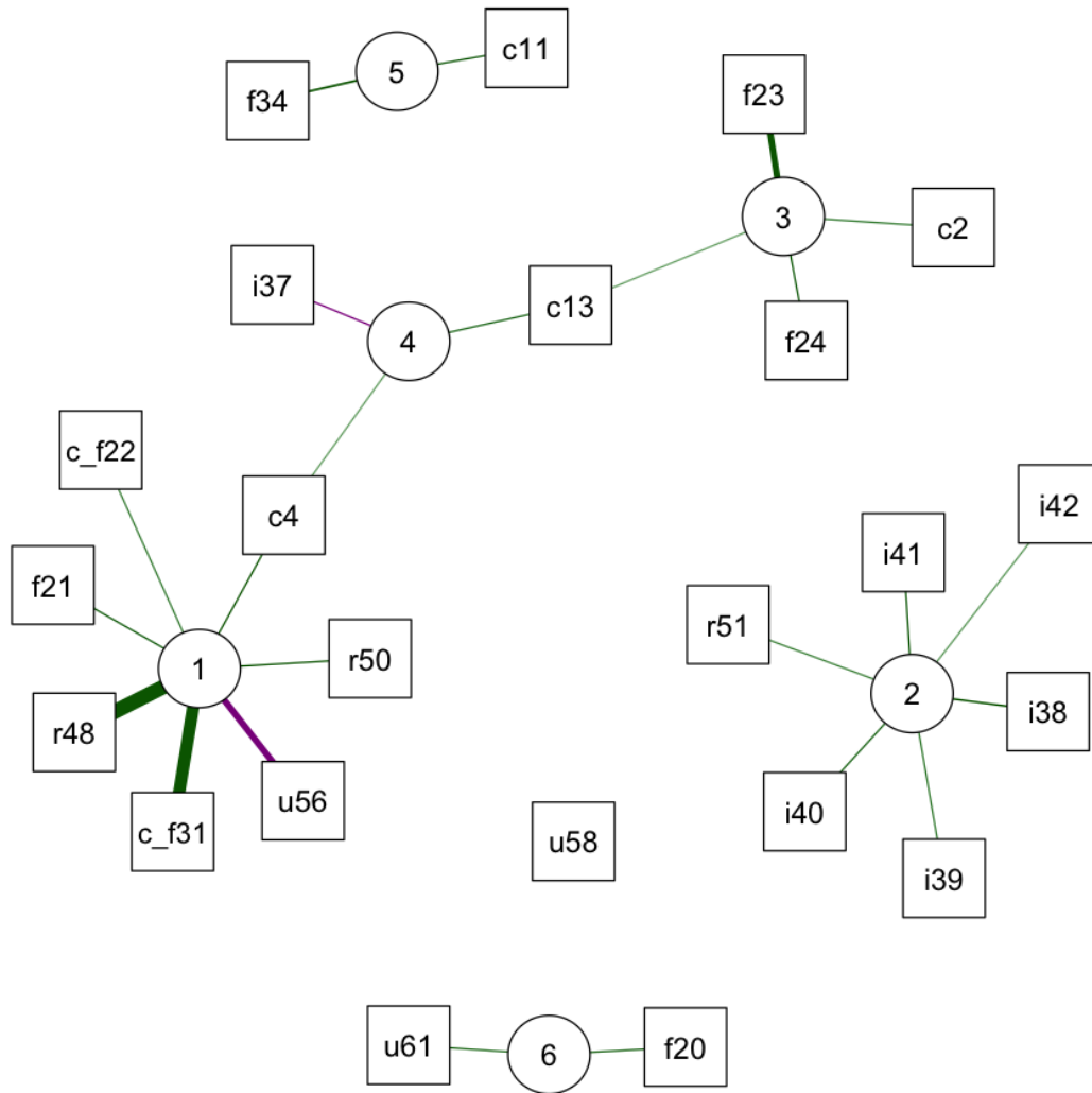
Figure 4.5: Loadings of individual indicators on principal components. The definitions of abbreviations for individual indicators are provided in Tables 4.1, 4.2, 4.3, 4.4, 4.5, pages 54-58. Indicators whose abbreviation begins with a letter followed by an underscore (e.g., c_f22) are those that changed the dimension in the final theoretical framework. In the previously mentioned tables, they can be identified by the last part of the abbreviation, i.e., the part after the underscore (e.g., f22).
