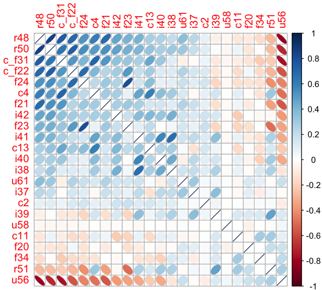
Figure 4.3: Correlations between the individual indicators. The definitions of abbreviations for individual indicators are provided in Tables 4.1, 4.2, 4.3, 4.4, 4.5, pages 54-58. Indicators whose abbreviation begins with a letter followed by an underscore (e.g., c_f22) are those that changed the dimension in the final theoretical framework. In the previously mentioned tables, they can be identified by the last part of the abbreviation, i.e., the part after the underscore (e.g., f22).
